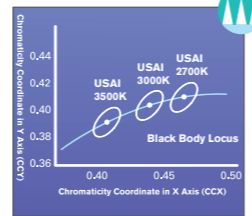
2-Step MacAdam Ellipse for Fixture-to-Fixture Color Consistency
