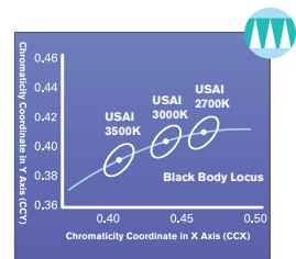
2-Step MacAdam Ellipse for Fixture-to-Fixture Color Consistency
